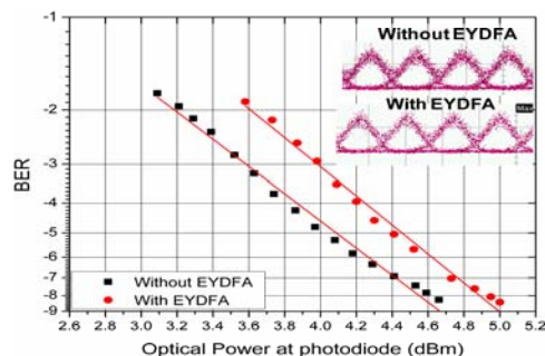
Fig. 3. Bit error ratio and eye diagrams (inset) at 40 Gb/s with and without the EYDFA in the communication link.
