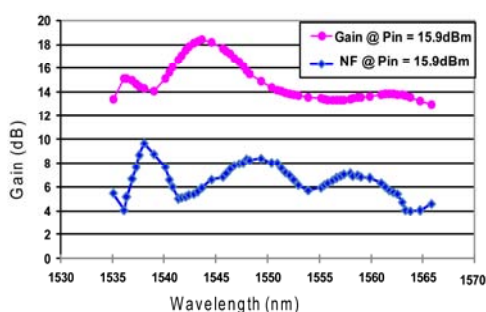
Fig. 2. Gain and Noise Figure (NF) of the EYDFA alone with input power to EYDFA ( P_{in} ) = 15.9 dBm
