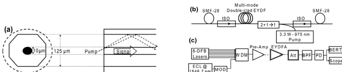
Fig. 1. Schematics of (a) the EYDF, (b) the EYDFA, and (c) the bit error ratio measurement setup. Mod: modulator, WDM: wavelength division multiplexer. BPF: bandpass filter@1546.7 nm, Att: variable attenuator, PD: Photodiode, BERT: BER tester.
