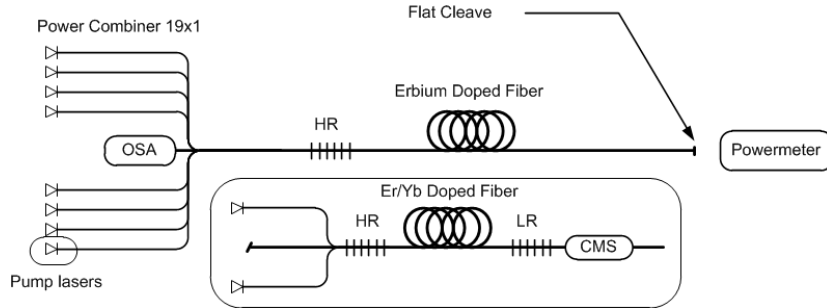
Fig. 1. Experimental setup
